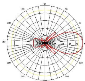
YA9-13 E Plane
