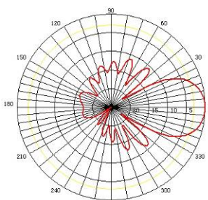
YA9-13 H Plane
