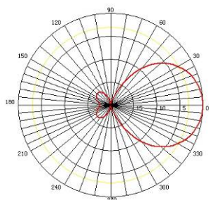
YA9-9 E Plane
