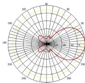
YA9-11 E Plane
