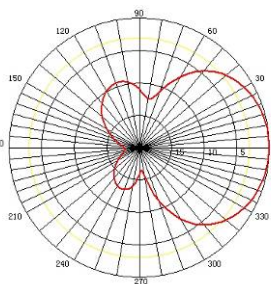
YA9-9 H Plane
